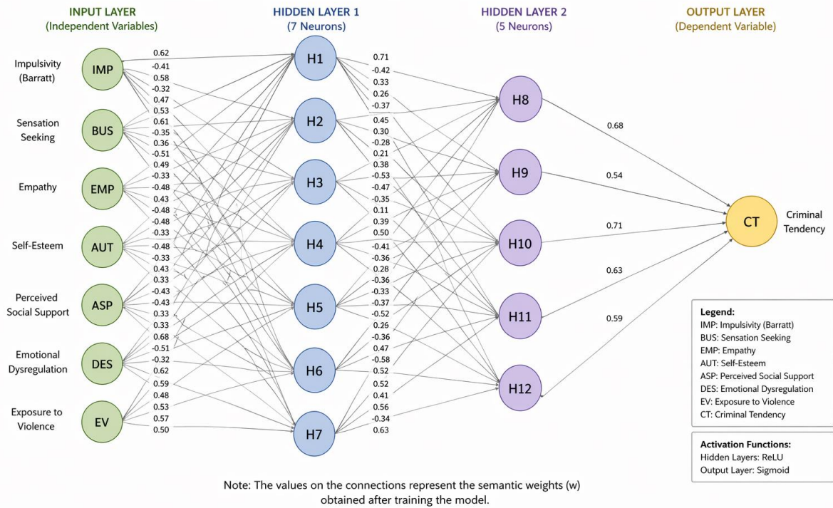
Fig. 1. Artificial Neural Network
